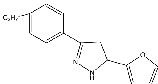
5-(furan-2-yl)-4,5-dihydro-3-(4-propylphenyl)-1H-pyrazole
