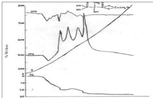
Fig 1: Derivatogram of Cu-HEDP-2H 2 O (100 mg specimen) Temperature, °C
