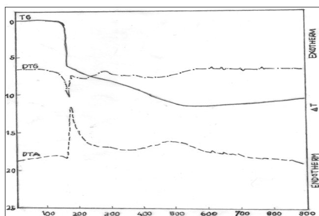
Fig 2: Thermoanalytical curves of Cu 5 (C 3 H 4 NO 8 P 2 ) 24 .H 2 O (200 mg specimen)
